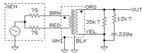
TEST CIRCUIT 2
