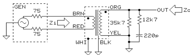
TEST CIRCUIT 1
